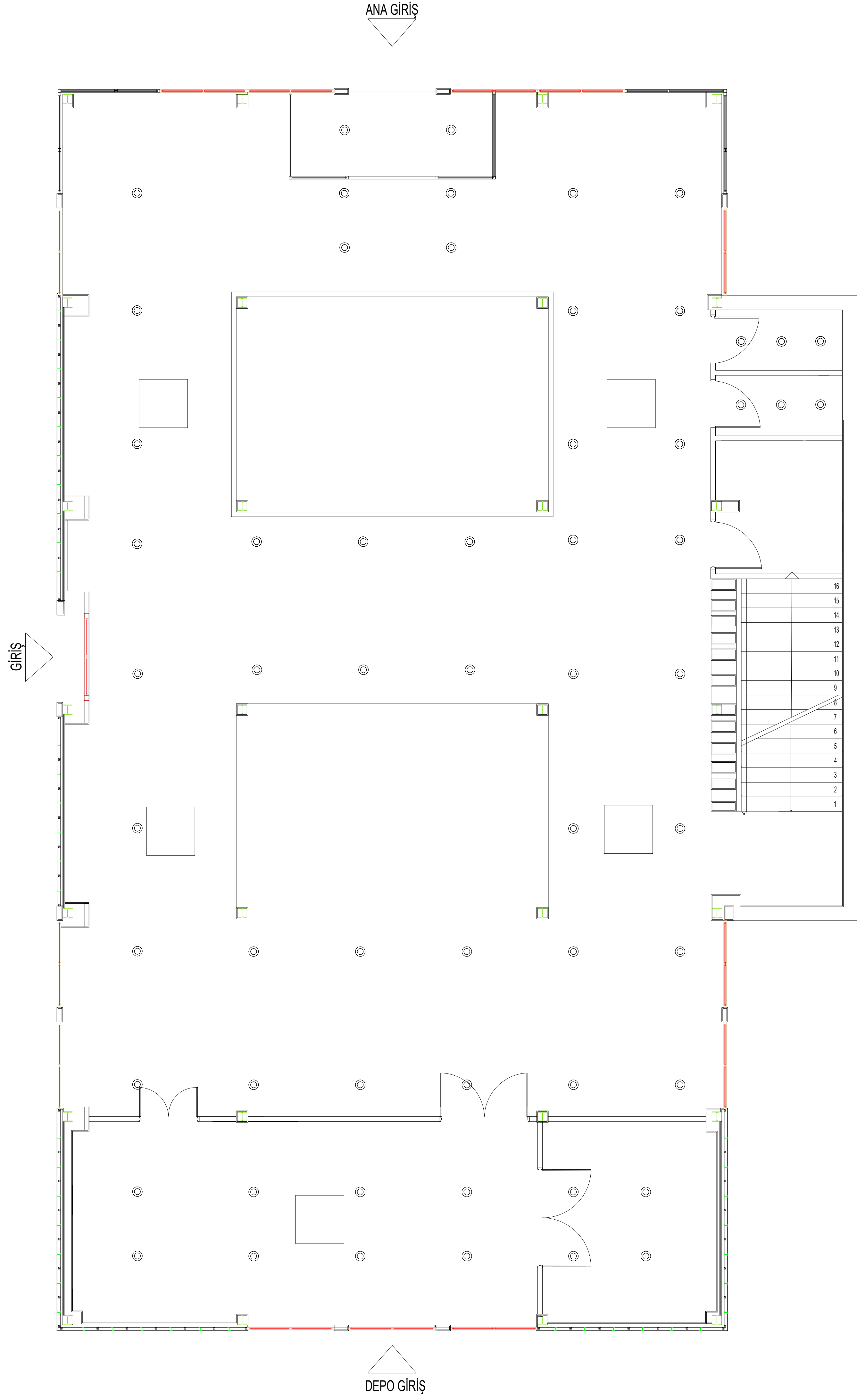
TAVAN PLANI 1/50
