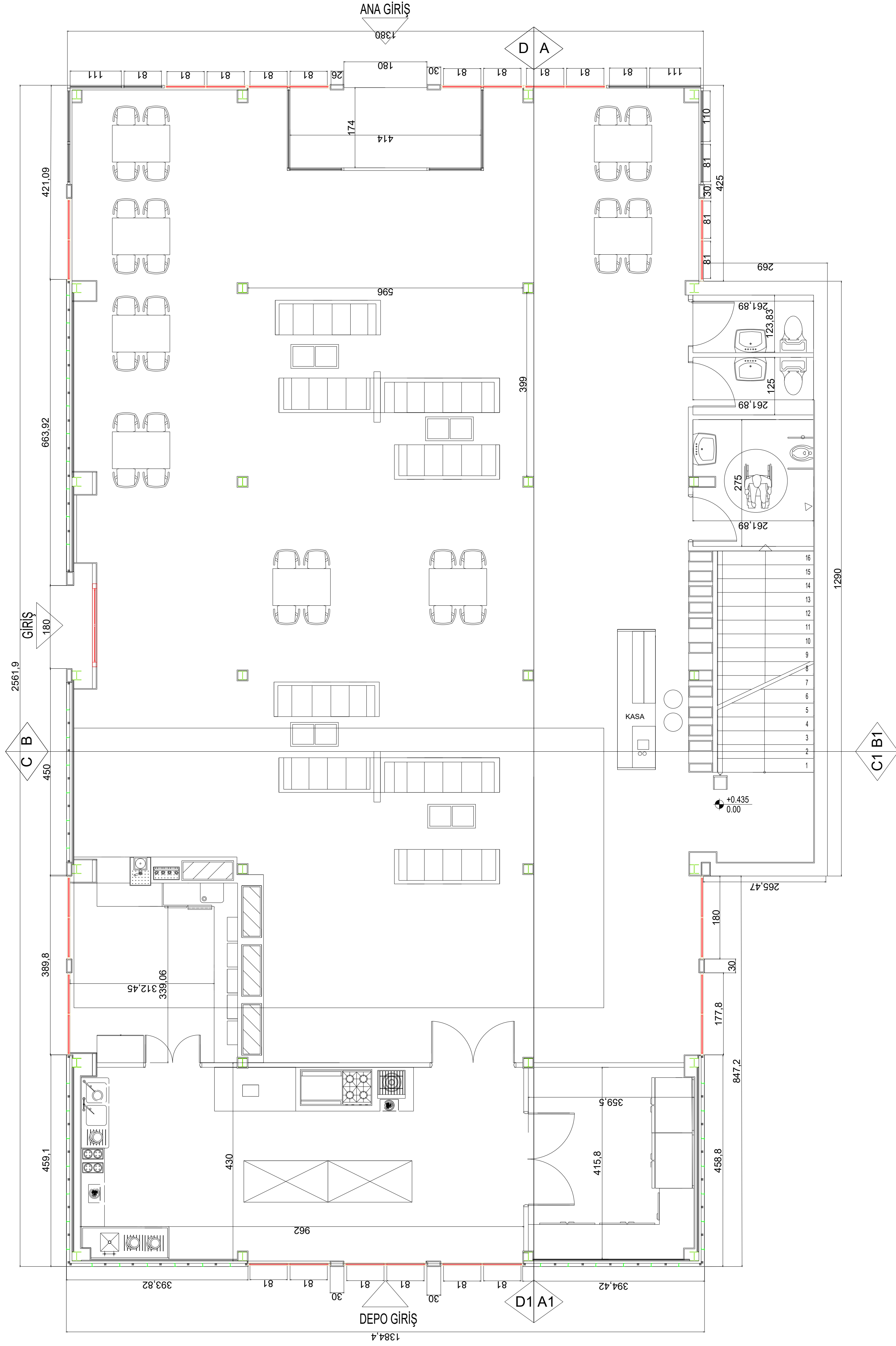
ZEMİN KAT PLANI 1/50
